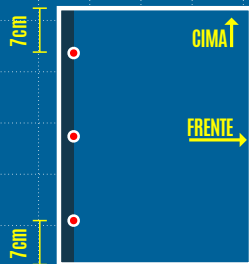
Lateral 2 (30x40cm) 3 furos
